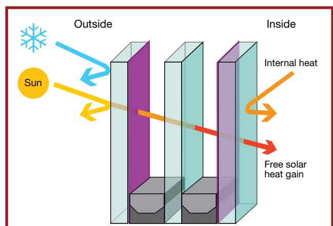
Figure 2: Triple glazing unit with two Low-E coatings
